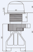
F款b型罩面防爆信号灯 F type b series cover face explosion-proof signal lamp
